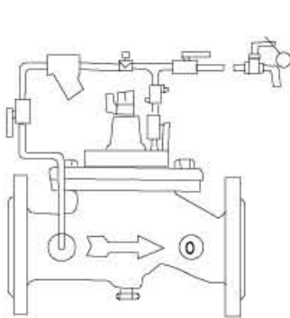
FIG: FS100X 遙控浮球閥
